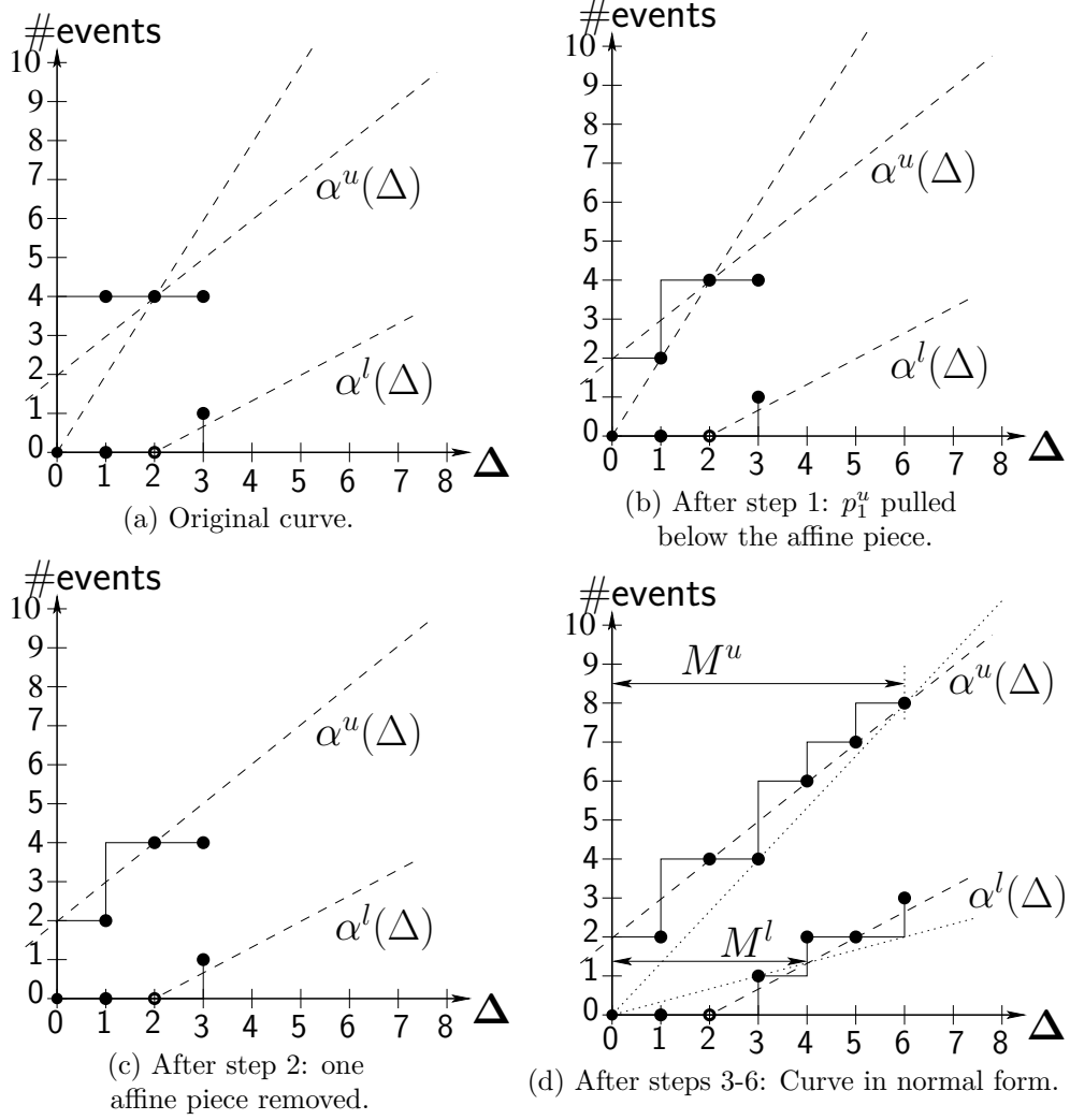
Figure 4: Step by step transformation into normal form
