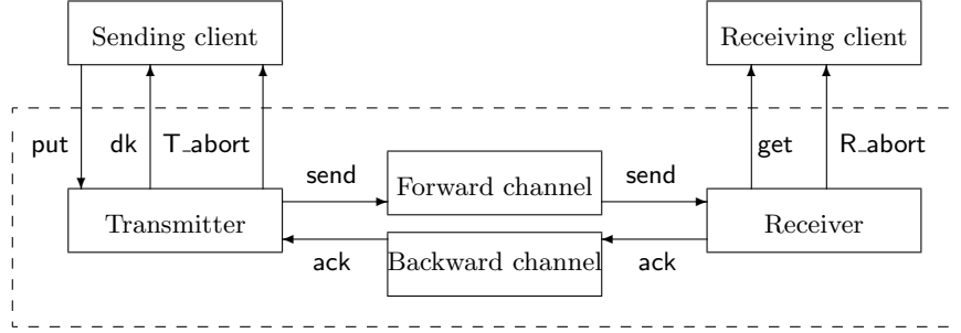
Figure 28: The BRP specification and interfaces
