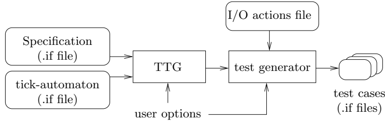
Figure 24: The TTTG tool.
