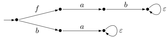
Figure 3. The automaton \mathcal{B}
