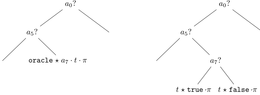
Figure 6.1: Harnessing the premise into a direct program.
