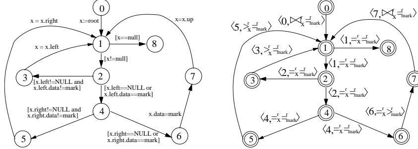
Fig. 4. The Depth-first tree traversal procedure and its initial abstraction
