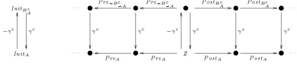
Figure 8: Commuting diagram for compact rectangular zones Z of a compact initialized rectangular automaton A
