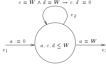
Figure 16: Equality lemma: testing if c = d
