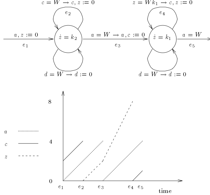
Figure 19: Counter increment: multiplying c by \frac{k_2}{k_1} using the two-slope variable z
