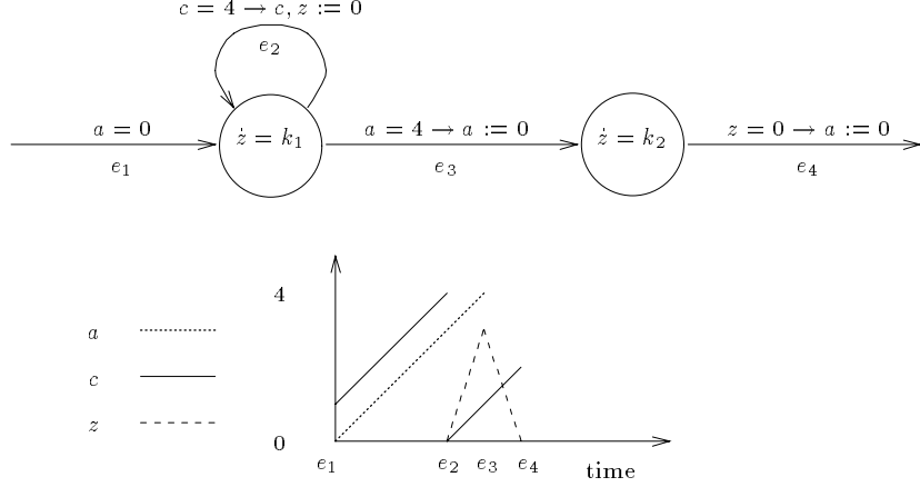
Figure 22: Doubling c when k_2 = -k_1
