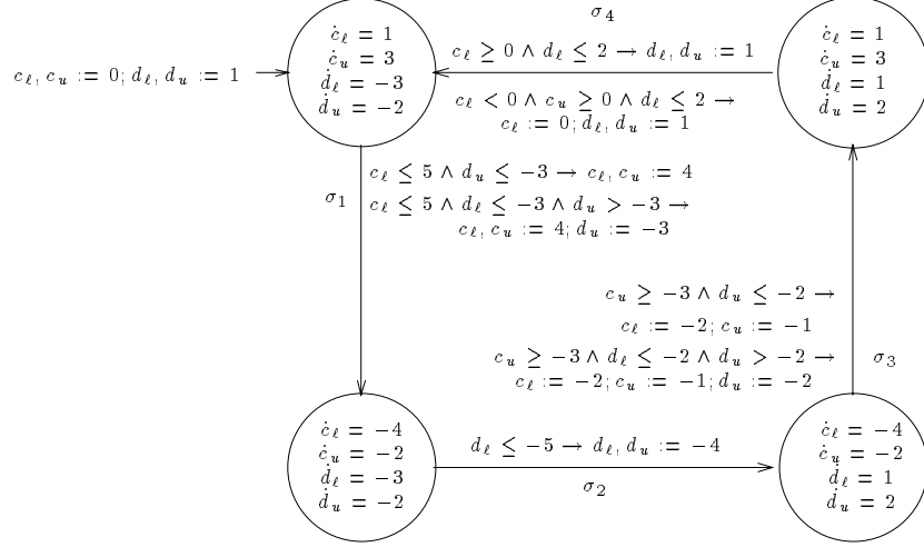
Figure 6: The initialized singular automaton B_{\hat{A}}^c
