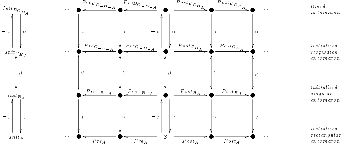
Figure 12: Putting together the commuting diagrams
