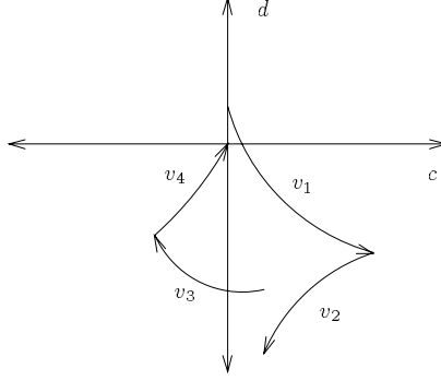
Figure 2: A sample trajectory of \hat{A}
