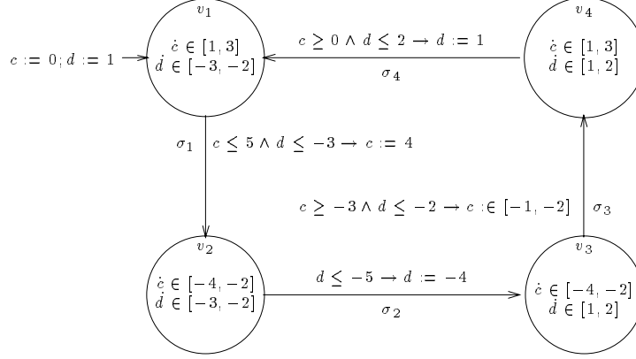
Figure 1: The initialized rectangular automaton \hat{A}
