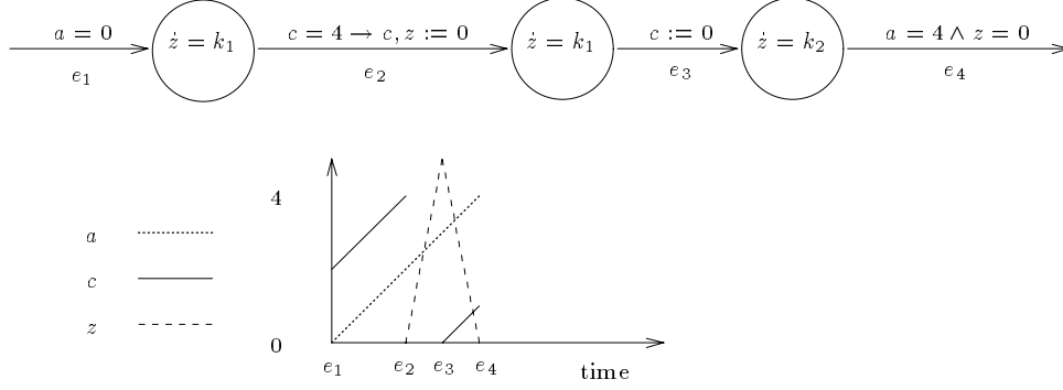
Figure 23: Halving c when k_2 = -k_1
