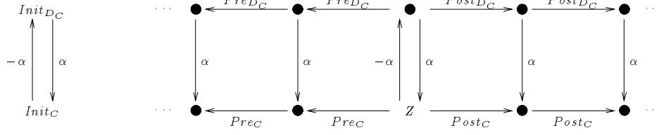
Figure 3: Commuting diagram for zones Z of an initialized stopwatch automaton C
