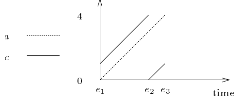
Figure 15: Proof of the wrapping lemma for slope 1
