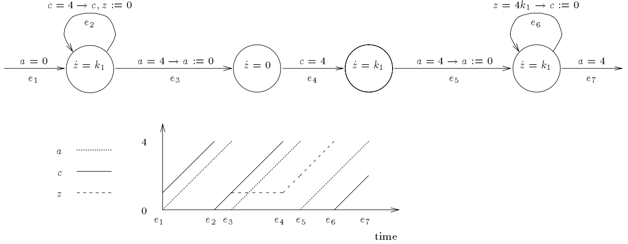
Figure 20: Doubling c using the two-slope variable z with the slopes 0 and k_1
