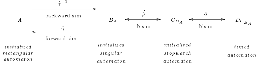
Figure 11: Chain of timed simulations from A to D_{C_{B_A}}
