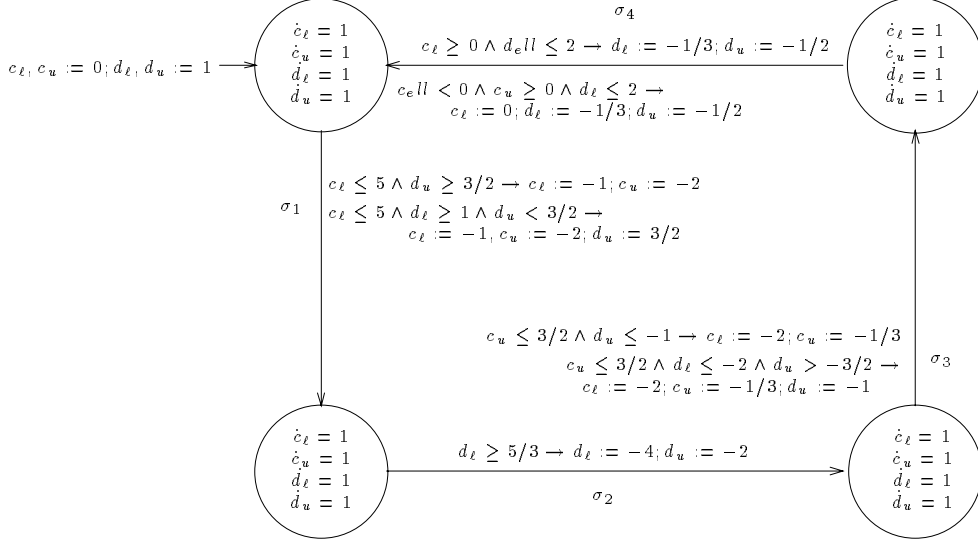
Figure 7: The initialized stopwatch automaton (and timed automaton) C_{B_A^c}
