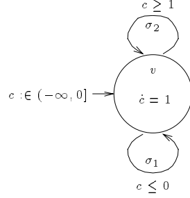
Figure 9: The initialized rectangular automaton \tilde{A} with Lang(\tilde{A}) \not\subseteq Lang(B_{\tilde{A}})
