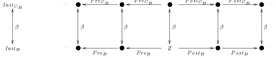
Figure 4: Commuting diagram for zones Z of an initialized singular automaton B
