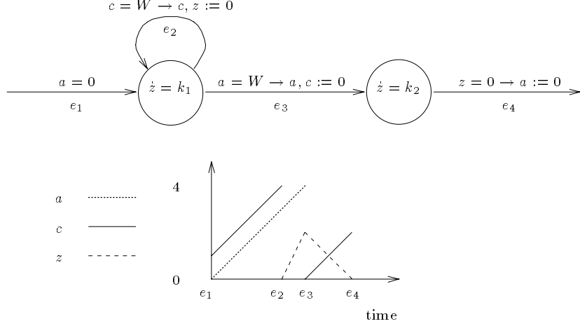
Figure 21: Multiplying c by \frac{k_1}{|k_2|} when k_1 > 0 > k_2 and |k_2| < k_1
