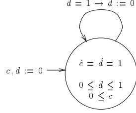
Figure 13: The timed automaton \hat{B} for which Reach(\hat{B}) \supseteq Post^i(Init) for all i \geq 0
