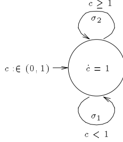
Figure 10: The initialized rectangular automaton \bar{A} for which \text{Lang}^c(\bar{A}) is not limit-closed
