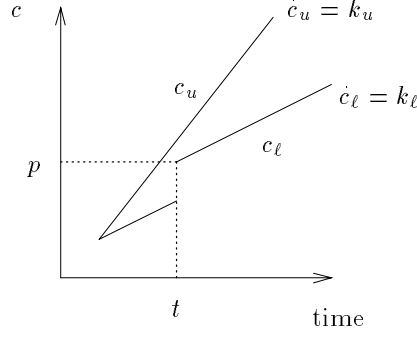
Figure 5: Envelope created by the flow interval flow(v)(c) = [k_\ell, k_u]
