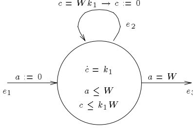
Figure 14: Wrapping lemma: the skewed clock c retains its entry value upon exit
