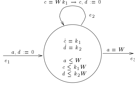
Figure 17: Assignment lemma: performing the assignment d := \frac{k_2}{k_1} \cdot c
