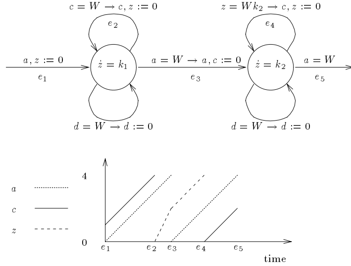
Figure 18: Counter decrement: multiplying c by \frac{k_1}{k_2} using the two-slope variable z
