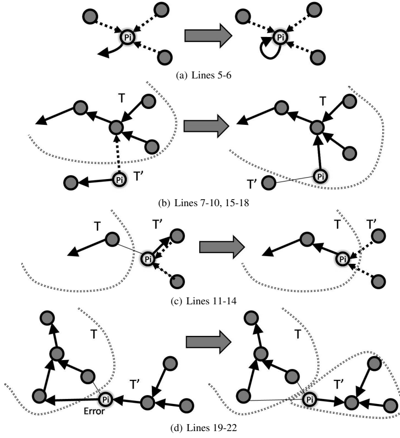
Fig. 3 Outline of the proposed algorithm
