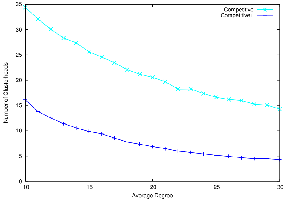
Figure 9: Competitive v.s. Competitive+, for n = 1000 , k = 5 , and a square field of size 4000m .
