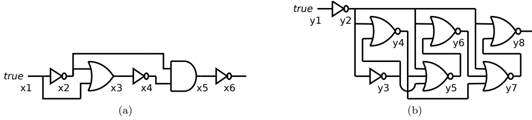
Figure 12: (a) The same Boolean circuit, and (b) its reduced form using Logic gates.
