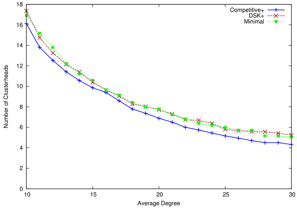
Figure 10: Competitive+ v.s. DSK+ v.s. Minimal, for n = 1000 , k = 5 , and a square field of size 4000m .
