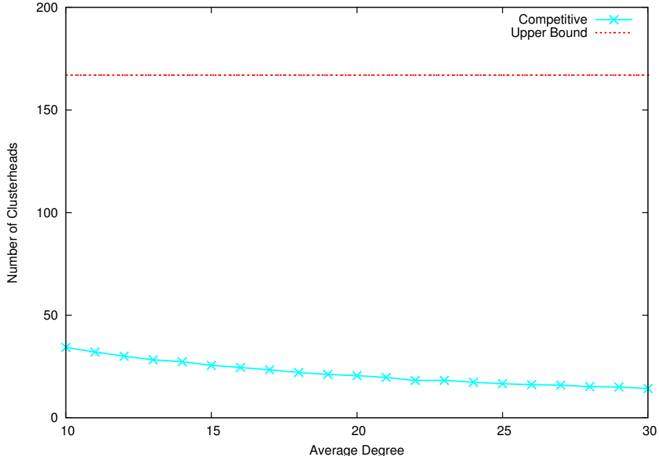
Figure 7: Competitive v.s. its theoretical bound \lceil \frac{n}{k+1} \rceil , for n = 1000 , k = 5 , and a square field of size 4000m .
