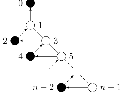
Figure 2: Worst case example for MIS tree height.
