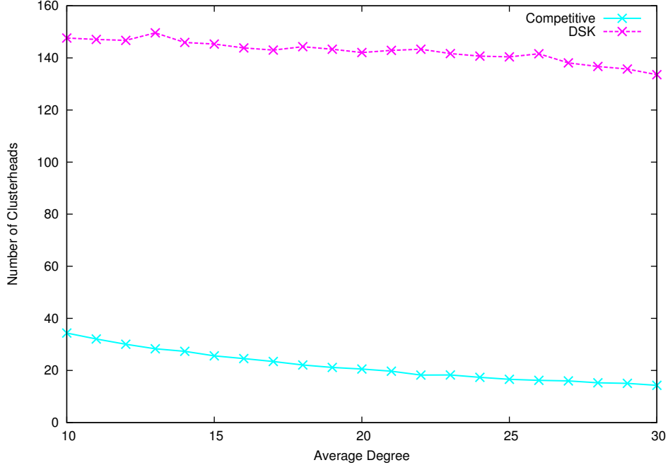
Figure 8: Competitive v.s. DSK, for n = 1000 , k = 5 , and a square field of size 4000m .
