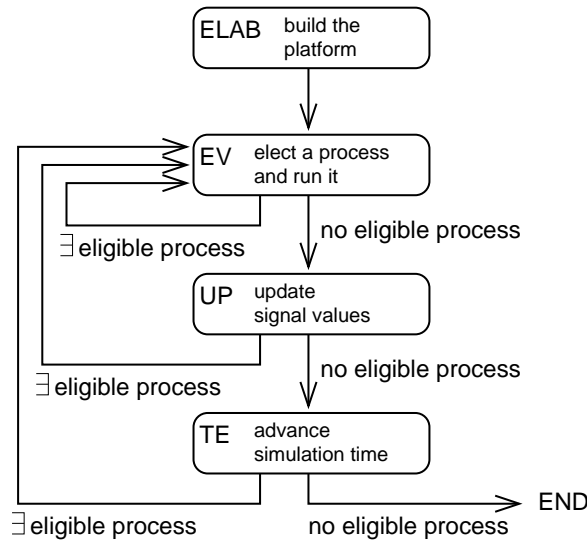
Figure 2: Automaton of the SystemC Scheduler
