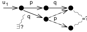
Figure 5: A Potential Divergent Path, black circles represent global states of the model
