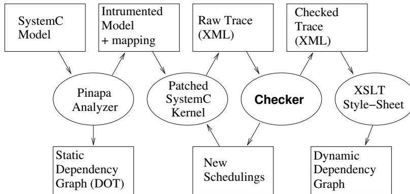
Figure 8: The Prototype's Architecture
