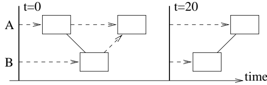
Figure 6: Dynamic Dependency Graph
