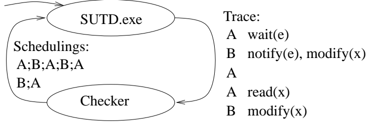
Figure 7: First iteration of the analysis for the \text{f}\circ\circ example. The first execution activates processes A and B in the order ABAAB . The checker generates two new schedulings. One to permute A_1 and B_1 (unordered accesses to event e ) and the other to permute A_3 and B_2 (unordered accesses to shared variable x ).
