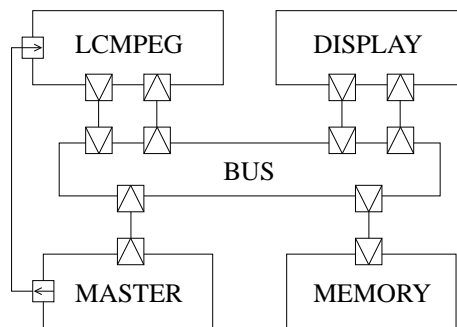
Figure 10: Architecture of the MPEG decoder system
