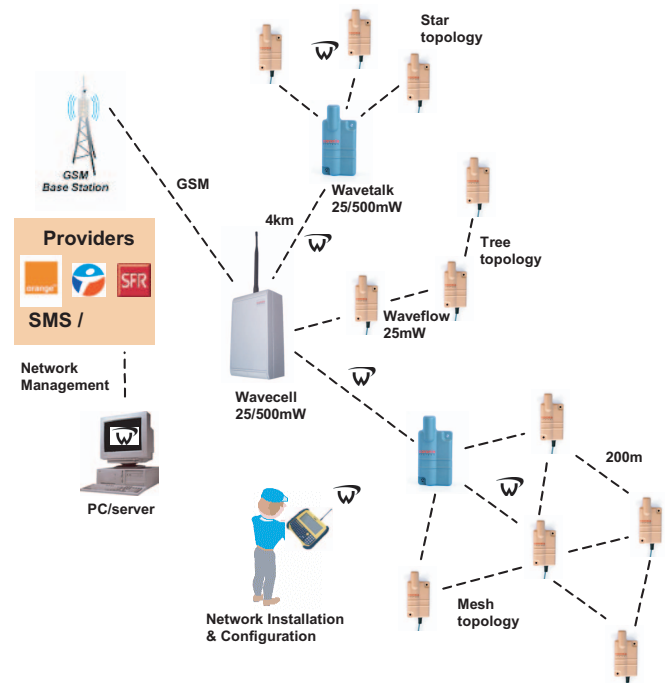
Fig. 2. An optimal topology is automatically configured for each local group in a large-scale ultra-low power network.
