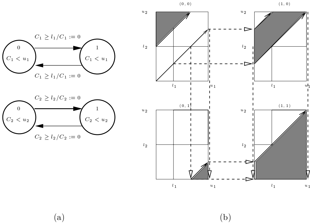
Figure 4: (a) Two TA representing two independent oscillators. (b) The first steps in computing all their possible behaviors. Dashed lines indicate discrete transitions.
