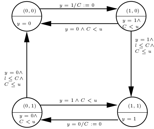
Figure 3: The timed automaton for a delay element. The runs of the automaton are exactly those satisfying y \in D_{[l,u]}(x) .
