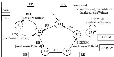
Figure 10. FIFO-Read component
