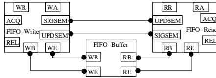
Figure 9. Low-level implementation BIP model for software channels
