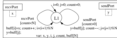
Figure 5. SW-channel (FIFO) in BIP
