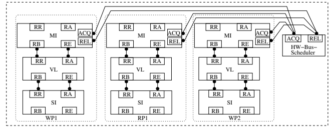
Figure 8. The BIP Model of the LB1 bus
