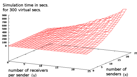
Figure 6. SenderReceiver example.
