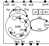
Figure 2. A nesC module in BIP.
