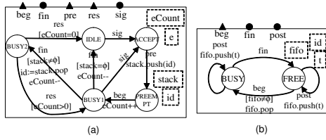
Figure 3. Event(a) and Task(b) Schedulers.
