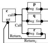
Figure 4. Connectors for a nesC call.
