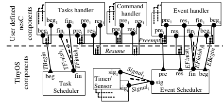
Figure 5. The global architecture in BIP.
