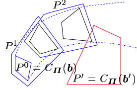
Fig. 1. Illustration of the computation of continuous successors. After two iterations new abstract state (l, \mathbf{b}') is reachable.
