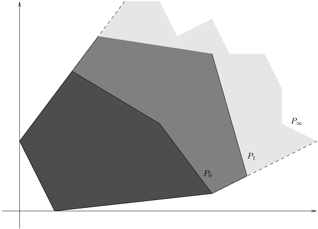
Figure 3: The standard widening on convex polyhedra [36, 58], here demonstrated on polyhedra in dimension 2 (polygons). The widening operator observes the sets of reachable states P_0 and P_1 at two consecutive iterations, and keeps only the constraints (polyhedral faces, here polygon edges) that are stable across iterations. The resulting P_\infty polyhedron is then proposed as an invariant.
